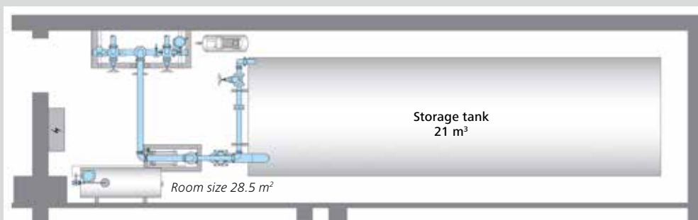
A Classic sprinkler pump room
